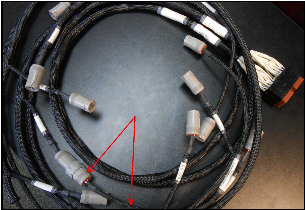
Harness shown with one jumper – see arrows The harness is shipped with ten jumpers (one jumper serves two cylinders)
